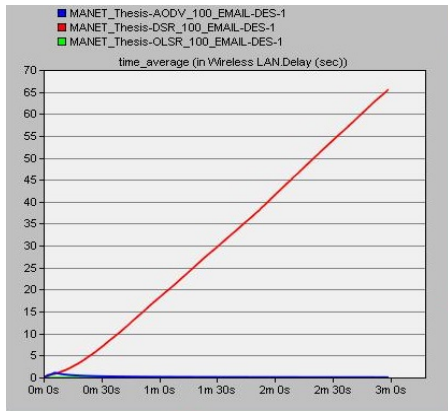
Fig 3: Delay comparison in three routing protocols for 100 nodes
