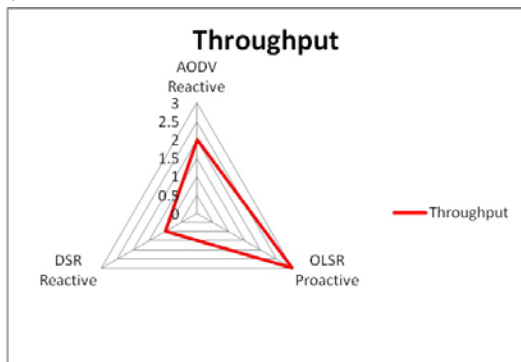
Fig 4. KIVIAT diagram with “throughput” for AODV, OLSR and DSR routing protocols comparison
