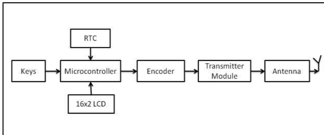
Fig. 5: Block Diagram of Transmitter Section
