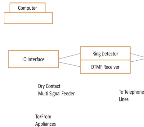
Fig. 3: Smart control system to control a appliances remotely by phone
