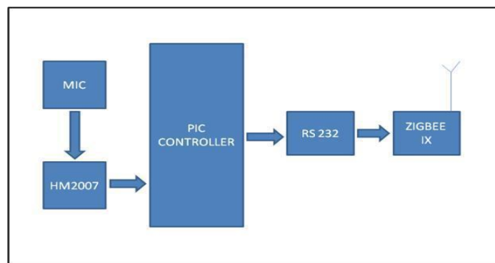
Fig. 4: Block Diagram of Transmission Unit
