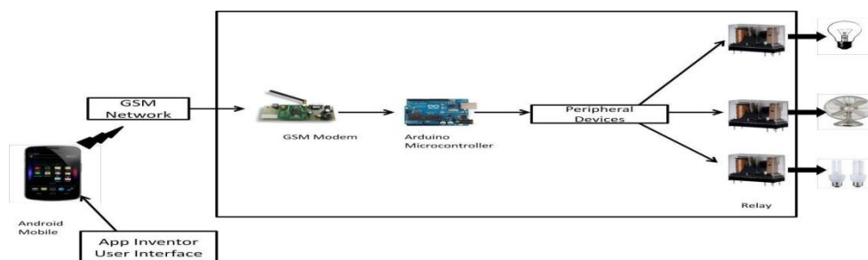
Fig. 1: GSM based HAS
