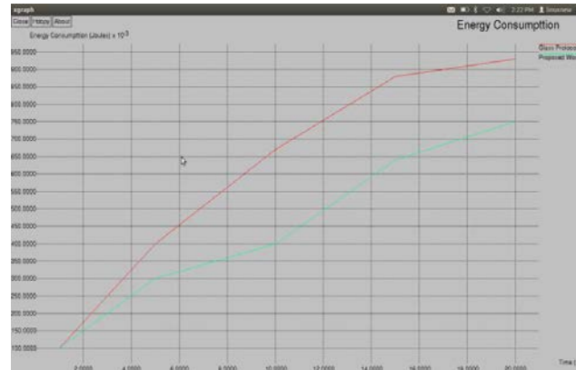
Fig 4: Comparison of proposed scheme and GLASS protocol in term of energy consumption
